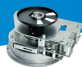
SS2-SD Manual Single-Spring Mechanism
