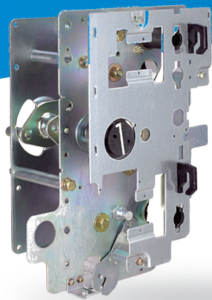
Manual Operating Mechanism ( For LBS ) Model: SPE02 -SJ Drawing No.: 3WXJ.085.001
