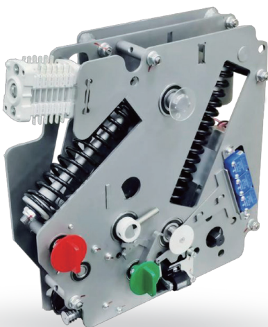
SPD31 Circuit Breaker Mechanism
