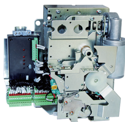
SPE203 Fuse switch Mechanism
