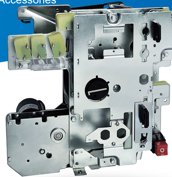
Motorized Operating Mechanism ( For Fuse-Switch )
