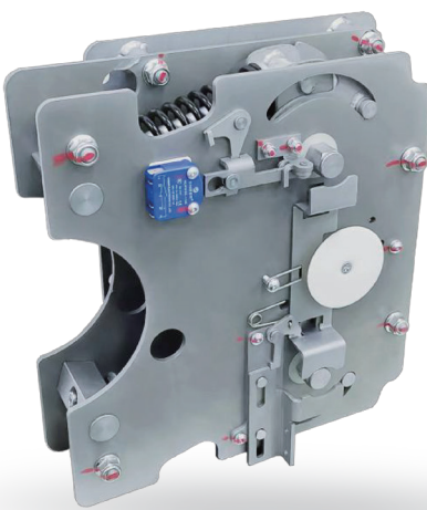
SPE31 Three-Position Switch Mechanism
