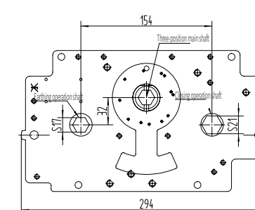
Mechanism front plate
