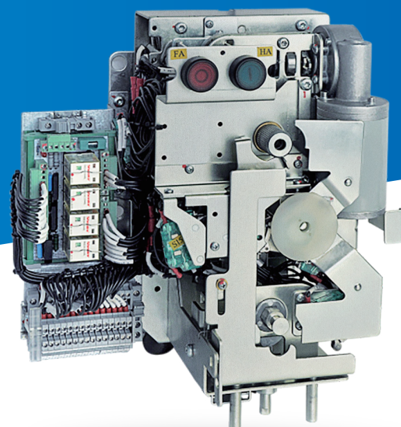
SPE203 Fuse switch Mechanism
