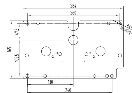
Base plate mounting position and overall dimensions
