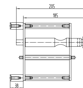
Height dimension
